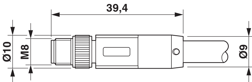
Dimensional drawing
